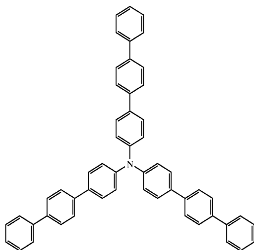
p-TTA (T g = 132° C.)
