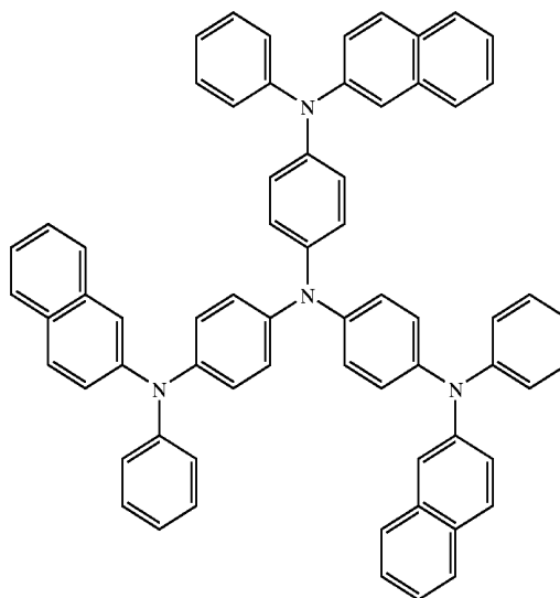
2-TNATA (T g = 110° C.)
